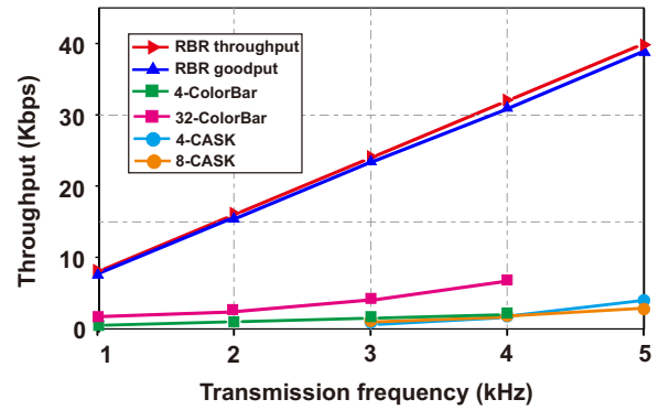
Fig. 13: Throughput improvement compared with state-of-art high-order modulation methods: ColorBar [7] and CASK [5].
